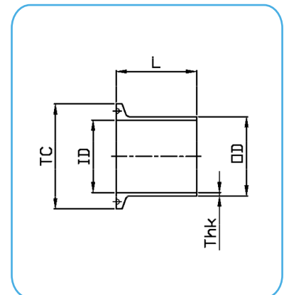
FERRULE CLAMP BS 4825
